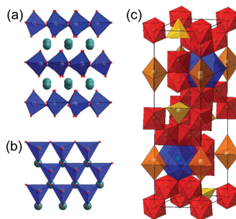
Fig. 3 Example of hexagonal ferrites (a) and (b) shows the \text{ABO}_3 hexagonal layered perovskite structure as found for \text{YbFeO}_3 ( \text{YMnO}_3 type), where [\text{BX}_6] trigonal bipyramids are shown in blue and layers of A cations are the green spheres: (a) view showing stacking of layers and (b) a view perpendicular to the layers. (c) shows the unit cell of the hexaferrite \text{BaFe}_{12}\text{O}_{19} with three distinct iron environments: octahedral (red), tetrahedral (yellow) and pyramidal (orange) and 12-fold coordination sites for Ba (blue).
