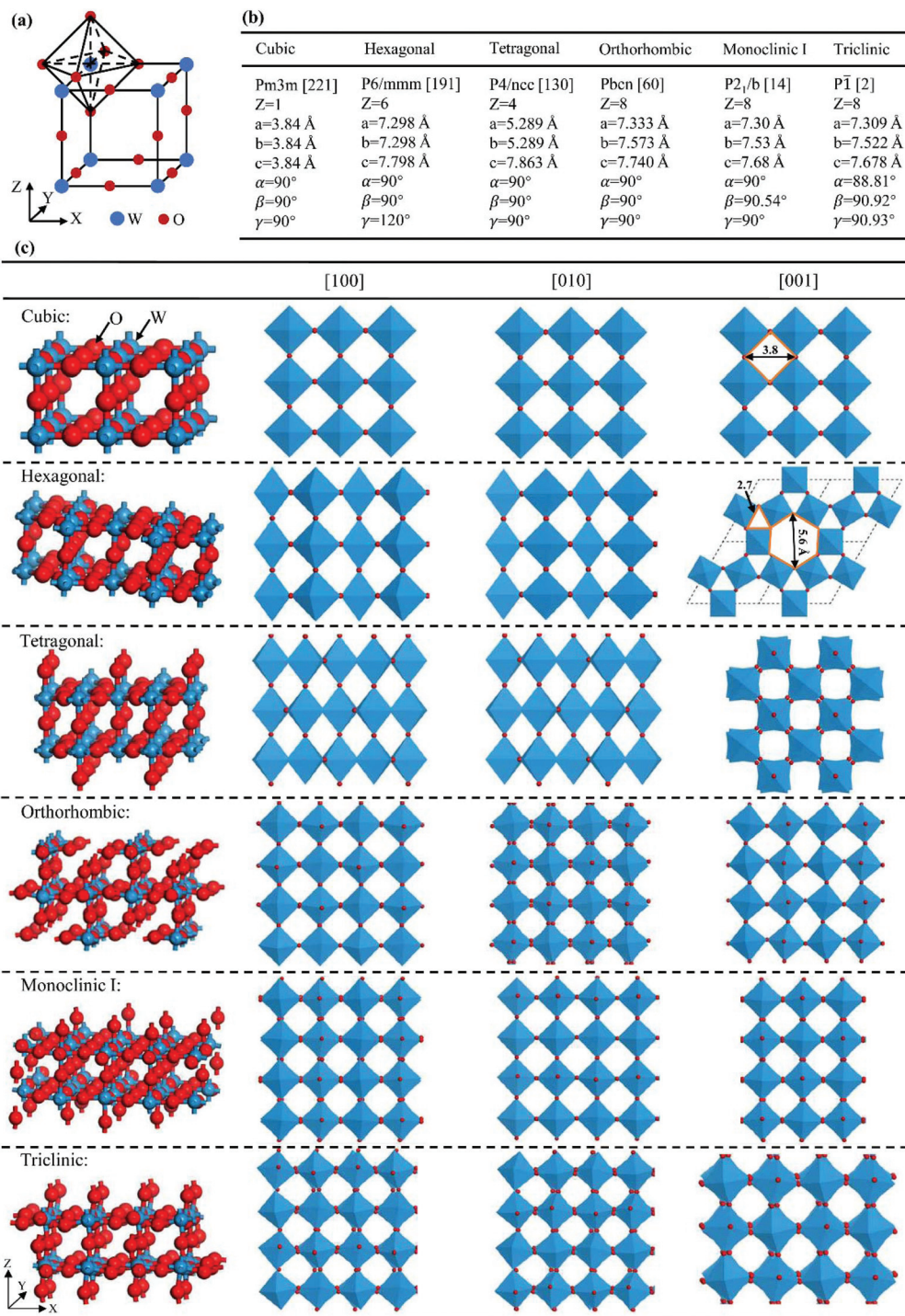
Fig. 5 Crystal structures of polymorphic WO 3 : cubic WO 3 and its WO 6 octahedron (a), structural parameters (b), and stick–ball and polyhedral representations (c).
