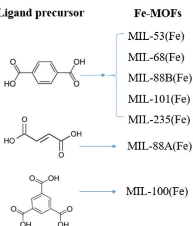
Fig. 4 (A) Fe-MOFs prepared with different ligand precursors; (B) structures of metal clusters and representative MIL series of Fe-MOFs. Adapted with permission from ref. 39, © 2018 WILEY-VCH.
