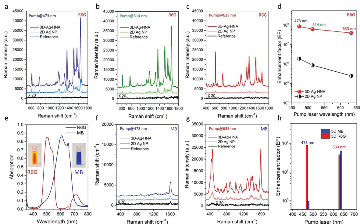
Fig. 5 SERS spectra measured from the R6G-treated 3D Ag HNA, conventional 2D Ag NPs and smooth Ag film (reference), the excitation laser wavelength is (a) 473 nm, (b) 514 nm and (c) 633 nm, respectively. (d) Enhancement factor of the 3D Ag hybrid nanostructure under different laser wavelengths. The laser power used on the 3D-Ag-HNA substrate was 100 \mu W, while on the 2D Ag NP substrate and the reference substrate the laser power was 1 mW. (e) Optical absorption of R6G and MB. SERS spectra measured from the MB-treated 3D Ag HNA, conventional 2D Ag NPs and smooth Ag film (reference), the excitation laser wavelength is (f) 473 nm and (g) 633 nm, respectively. (h) Calculated EF of R6G and MB on the 3D-Ag-HNA SERS substrate under different laser wavelengths.
