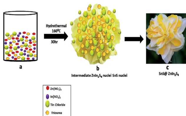
Scheme 1 Schematic of the formation mechanism of \text{SnS}@Z\text{nIn}_2\text{S}_4 nano-heterostructures.
