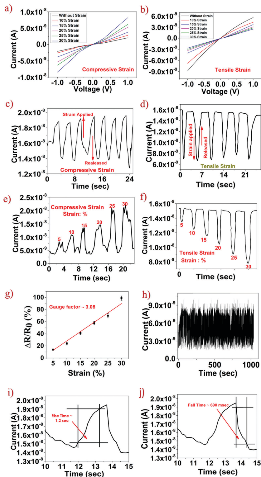
Fig. 4 (a and b) I-V characteristics of the Sn 2 S QD/PVA film under compressive and tensile strain respectively. (c and d) Continuous-time sensor response under constant compressive and tensile strains. (e and f) Temporal response of the sensor with an increase in compressive and tensile strains. (g) Graph showing the normalized resistance (%) vs. strain (%), gauge factor calculated to be \sim 3.08 . (h) Response of the fabricated sensor for 1000 strain cycles. (i and j) Rise time and fall time of the strain sensor were \sim 1.2 s and \sim 690 ms.
