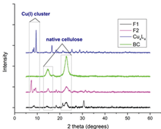
Fig. 1 X-ray diffractograms of papers F1 and F2, Cu(I) cluster ( \text{Cu}_4\text{L}_4 ) and bacterial cellulose (BC).
