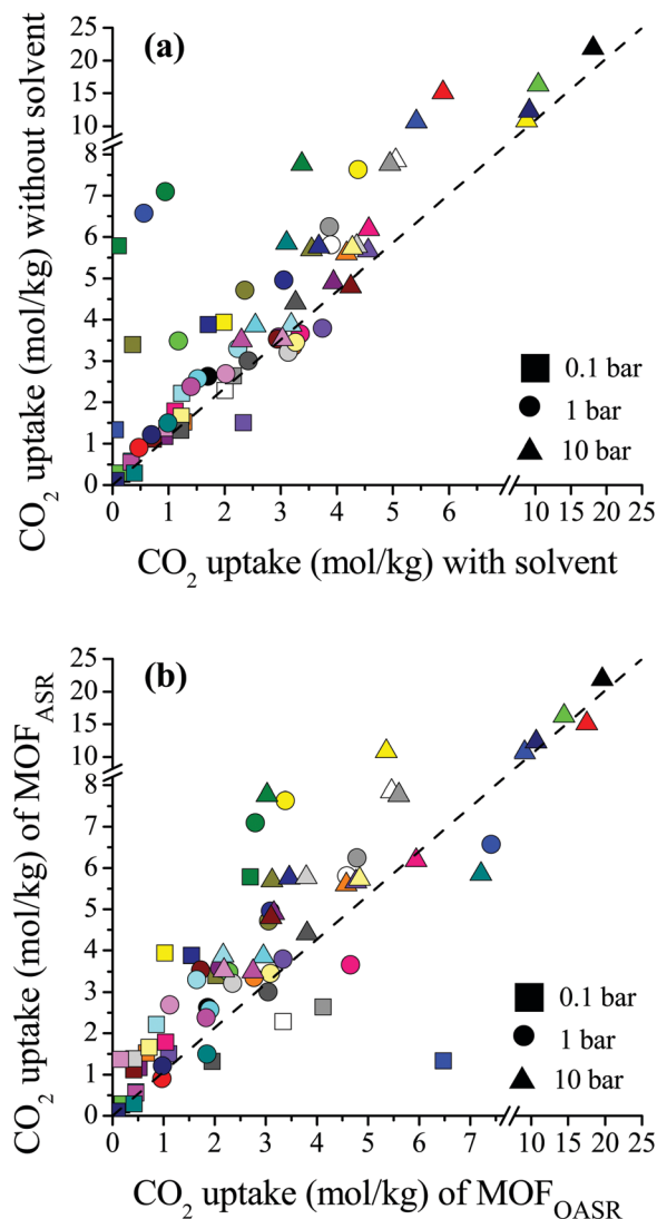
Fig. 1 (a) Comparisons of the single-component \text{CO}_2 uptakes of MOFs with and without coordinated solvent molecules. (b) Comparisons of the single-component \text{CO}_2 uptakes of MOFs after solvent removal ( \text{MOF}_{\text{ASR}} ) and MOFs optimized after solvent removal ( \text{MOF}_{\text{OASR}} ) at 0.1, 1 and 10 bar. Each MOF is represented with a different color. Detailed information about the refcodes of the MOFs, their solvent types and simulated \text{CO}_2 uptakes at different pressures is given in Table S1 (ESI†).
