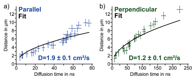
Fig. 4 (a) Diffusion times parallel to the domains derived from fits of time-resolved PL decays plotted versus the distance between detection and excitation with the data fit according to eqn (2) and the parallel diffusion constant. (b) Diffusion times perpendicular to the domains derived from fits of time-resolved PL decays plotted versus the distance between detection and excitation with the data fit according to eqn (2) and the perpendicular diffusion constant.
