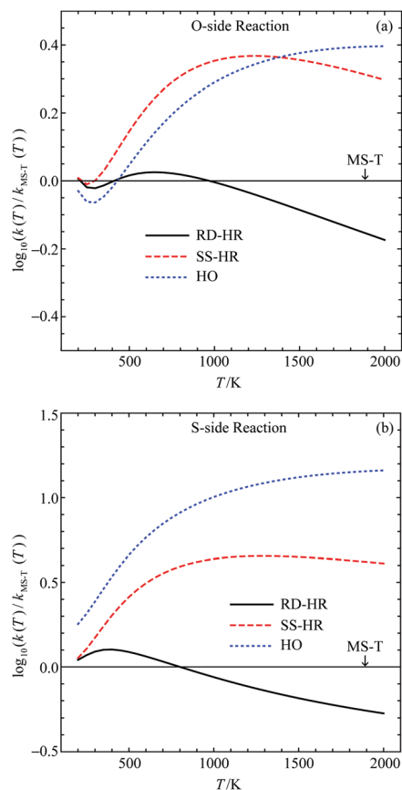
Fig. 4 Comparison of rate constants for (a) O-side and (b) S-side pericyclic H transfer reaction for O,S -diethyl methylphosphonothiolate calculated using various approximated hindered rotor models. The rate constants for the MS-T results, as well as the geometries, relative energies, vibrational frequencies and anharmonic constants of reactant and TS's can be found in ref. 22.
