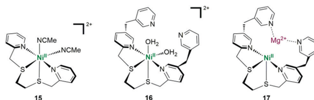
Fig. 14 Ni complexes for CO 2 photoreduction bearing an S 2 N 2 -type tetradentate ligand as the photocatalyst and a Ni(II) complex bearing an S 2 N 2 -tetradentate ligand with two noncoordinating pyridine pendants as the photocatalyst.
