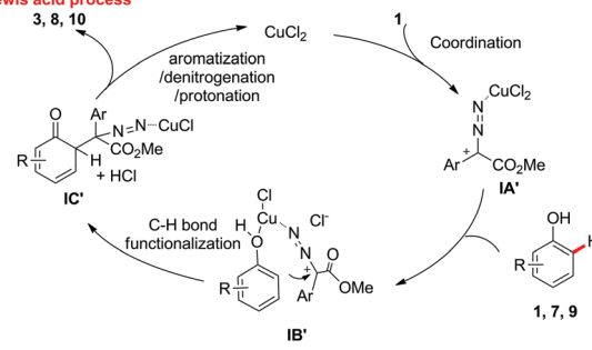
Scheme 6 Proposed catalytic cycle.
