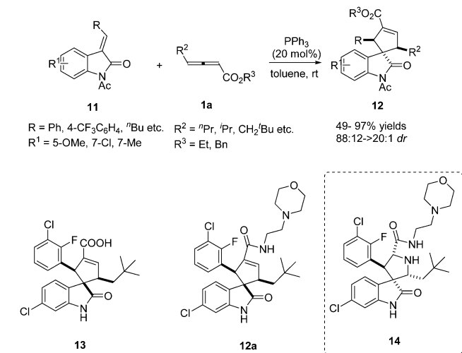
Scheme 4 Phosphine-catalysed (3+2) cycloaddition reactions of 3-benzylideneindolin-2-ones.
