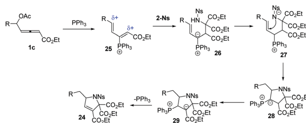
Scheme 8 Plausible mechanisms.
