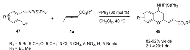
Scheme 14 Phosphine-catalysed abnormal (2+4) annulations of \gamma -methyl allenolate with N -thiophosphorylimines.
