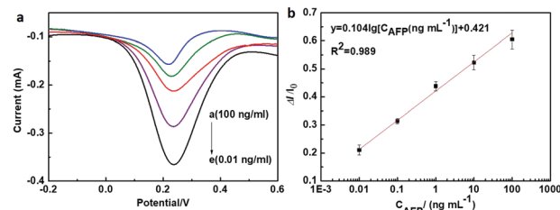
Fig. 5 (a) Differential pulse voltammetry of the as-prepared immunosensors in the presence of AFP with different concentrations (0.01 \text{ng mL}^{-1} , 0.1 \text{ng mL}^{-1} , 1 \text{ng mL}^{-1} , 10 \text{ng mL}^{-1} , and 100 \text{ng mL}^{-1} ). (b) Corresponding calibration curve for AFP detection, the error bars represent the standard deviation obtained from three measurements ( n = 3 ).
