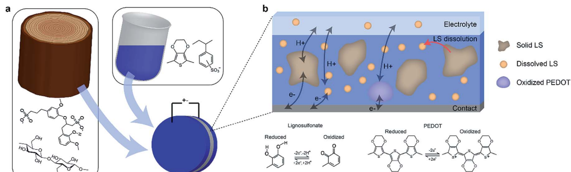
Fig. 1 Paper-based all-organic redox-enhanced supercapacitors. (a) The electrode is made up of nanofibrillated cellulose, PEDOT:PSS and lignosulfonate (LS). (b) Within the electrode, the LS is initially immobilized in its solid form during drying. Once the electrode is in contact with aqueous electrolyte, the solid LS can dissolve. The PEDOT and both solid and dissolved forms of LS participate in the electrode redox reactions.
