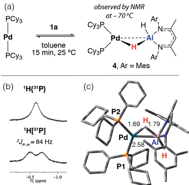
Scheme 2 (a) Reversible reaction of 1a with [\text{Pd}(\text{PCy}_3)_2] . (b) Hydride region of the ^1\text{H} NMR spectrum at -70^\circ\text{C} in toluene- d_6 . (c) Calculated structure of 4 with selected bond lengths in Å.
