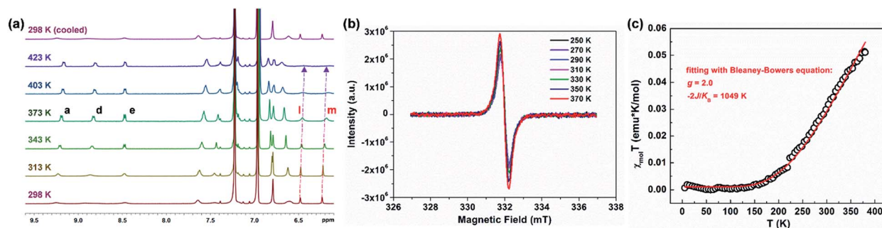
Fig. 2 (a) VT ^1H NMR experiment of 2 in o-C_6D_4Cl_2 . (b) EPR spectrum of a powdered sample of 2 recorded at 250–370 K. (c) SQUID measurement of a powdered sample of 2 from 5 to 400 K, experimental data plotted as black “O” and fitted curve according to the Bleaney-Bowers equation with g_e = 2.00 as a red line.
