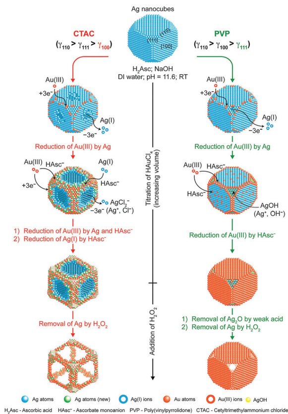
Fig. 7 Schematic illustration describing the mechanisms proposed for the deposition of Au and Ag atoms on Ag NCs when H_2AuCl_4^- is titrated into an aqueous suspension of Ag NCs in the presence of H_2Asc , NaOH, and CTAC (left) or PVP (right) at an initial pH of 11.6. Adapted with permission from ref. 101. Copyright 2017, American Chemical Society.
