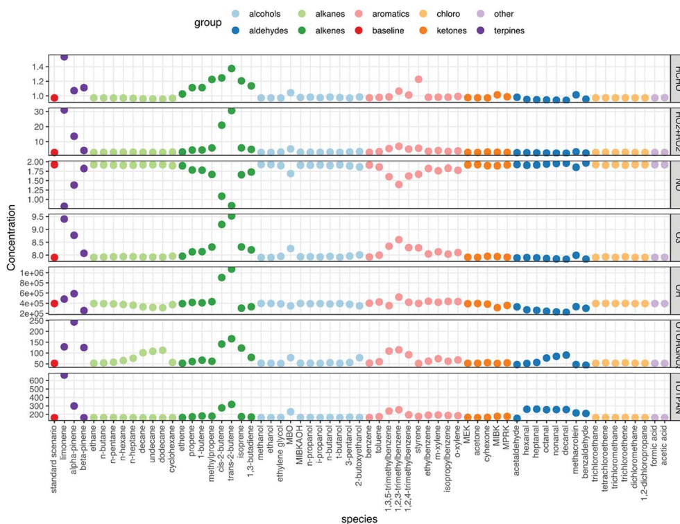
Fig. 2 Changes in mixing ratio for HCHO (ppb), \sum HO 2 + RO 2 (ppt), NO (ppb), O 3 (ppb), \sum organic nitrate species (ppt) and \sum PAN species (ppt) and concentration of OH (molecule per cm 3 ), with the addition of 10 ppb of different VOCs in turn. The molecules are colour coded according to functionality (see legend) and the standard run (with no VOCs added indoors) is shown in red.
