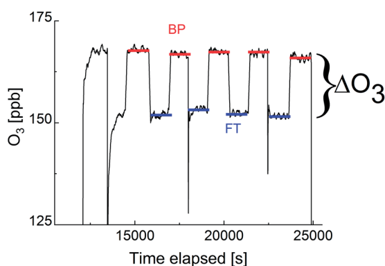
Fig. 2 An example of the O 3 mixing ratio measured downstream of the flow tube in response to switching the gas flow from the bypass (BP, red lines) to the injector and thus, through the coated wall flow tube (FT, blue lines). Experiments were done at 5 °C with an activity of Br - of 0.58 M and of citric acid of 0.08 M.
