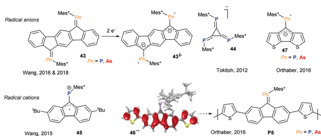
Fig. 12 Phospho- and arsaalkene-based radicals and radical reactions.
