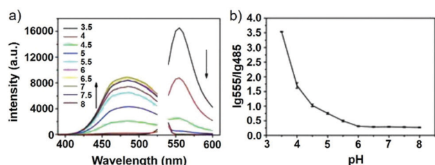
Fig. 19 pH dependent ratiometric fluorescence emission of probe 15 . (a) Fluorescence emission spectra of probe 15 (10 \mu\text{M} ) at pH 3.5–8.0 under dual-wavelength excitation ( \lambda_{\text{ex}} at 300 nm for dansyl group, 532 nm for R6G-lactam). (b) pH titration curves of lg ratios between fluorescence emission of R6G-amide ( I_{555\text{nm}} ) and that of dansyl group ( I_{485\text{nm}} ). Copyright 2013 Elsevier.
