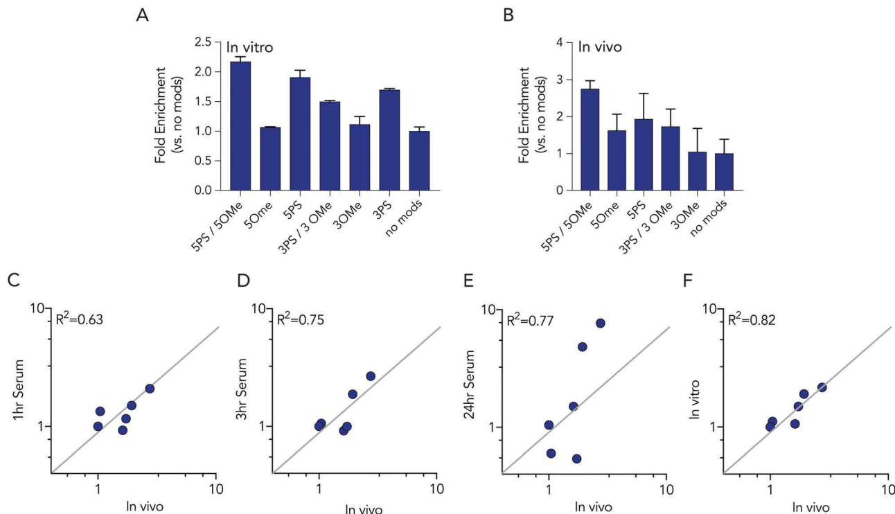
Fig. 5 Barcodes with 5 phosphorothioates and 5 2- O -methyl modifications exhibit increased stability in cells and in mice. (A) Enrichment of each DNA barcode compared to barcodes with no modifications in vitro in HEK293T cells at 24 hours. (B) Enrichment of each DNA barcode compared to barcodes with no modifications in vivo from lung endothelial cells at 24 hours. Correlation of in vivo enrichment compared to (C) 1 hour, (D) 3 hours, (E) 24 hours incubation in 10% mouse serum, and (F) in vitro in HEK 293T cells.
