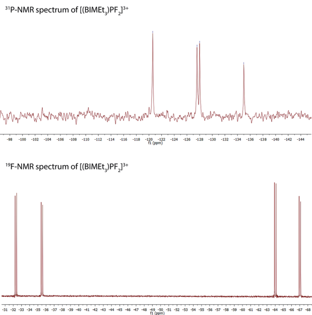
Fig. 3 NMR spectra for [PF 2 (BIMeEt 3 )] 3+ in CD 3 CN.
