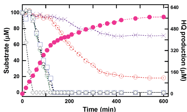
Fig. 1 Multiple turnover reactions of HadA with a mixture of para -substituted phenols. Multiple turnover reactions of HadA with a mixture of six substrates (100 μM each) including phenol (purple cross), 4-FP (empty red circle), 4-CP (empty blue square), 4-BP (empty green diamond), 4-IP (empty black triangle), and 4-NP (black plus) were carried out, and the amounts of products formed and substrates remaining were analyzed as a function of time. The amount of the product (HQ) formed is indicated by filled magenta circles.
