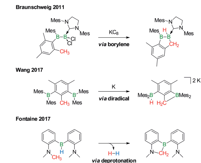
Scheme 2 Selected examples of transition metal-free intramolecular C(sp ^3 )-H activations through borylene (top), diradical (middle), and deprotonation reactions (bottom). Mes = 2,4,6-(H _3\text{C} ) _3\text{C}_6\text{H}_3 .
