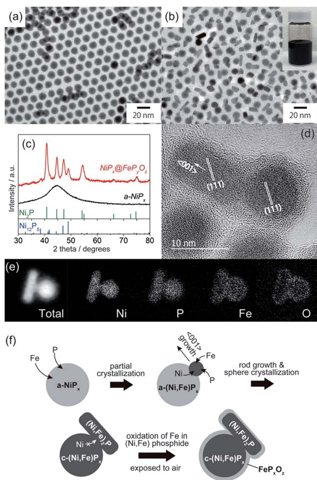
Fig. 1 TEM images of (a) a- \text{NiP}_x NPs and (b) \text{NiP}_x@FeP_yO_z NPs. The inset shows a hexane dispersion of the \text{NiP}_x@FeP_yO_z NPs stored for more than 6 months. (c) XRD patterns of a- \text{NiP}_x NPs and \text{NiP}_x@FeP_yO_z NPs. (d) HRTEM image of \text{NiP}_x@FeP_yO_z NPs. (e) STEM-EDS mapping images of a \text{NiP}_x@FeP_yO_z NP. (f) Schematic of the formation mechanism of \text{NiP}_x@FeP_yO_z NPs.
