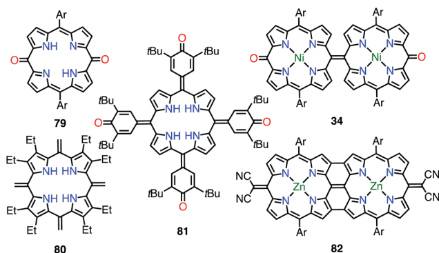
Fig. 26 Quinonoidal porphyrins.
