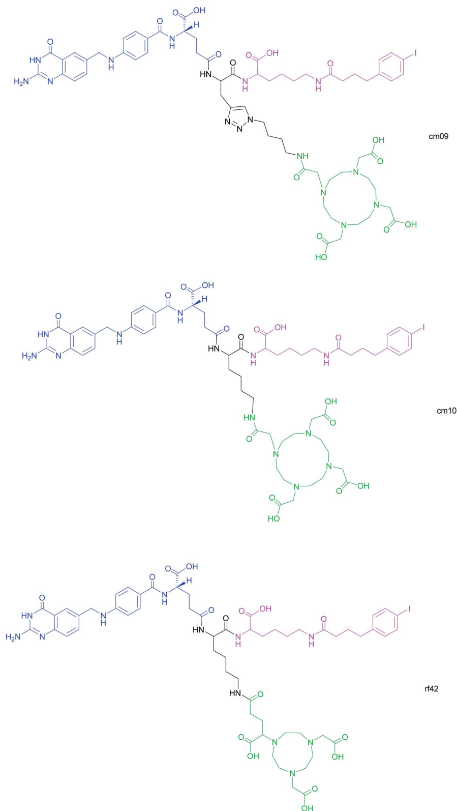
Fig. 16 Chemical structures of albumin-binding folate conjugates cm09, cm10 and rf42. They are each composed of three modules: (i) folic acid for \text{FR}\alpha -expressing tumour targeting (blue), (ii) an albumin-binding moiety (pink), and (iii) the chelator (green) (DOTA for cm09 and cm10 and NODAGA for rf42) for coordination of ^{68}\text{Ga} or ^{64}\text{Cu} . The three functionalities are connected via a lysine linker in radiofolates cm10 and rf42, and by a triazole linker in the case of conjugate cm09. 22,82,85
