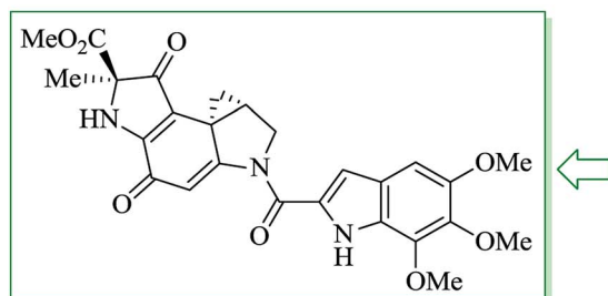
Scheme 92 Total synthesis of duocannycin A 436.
