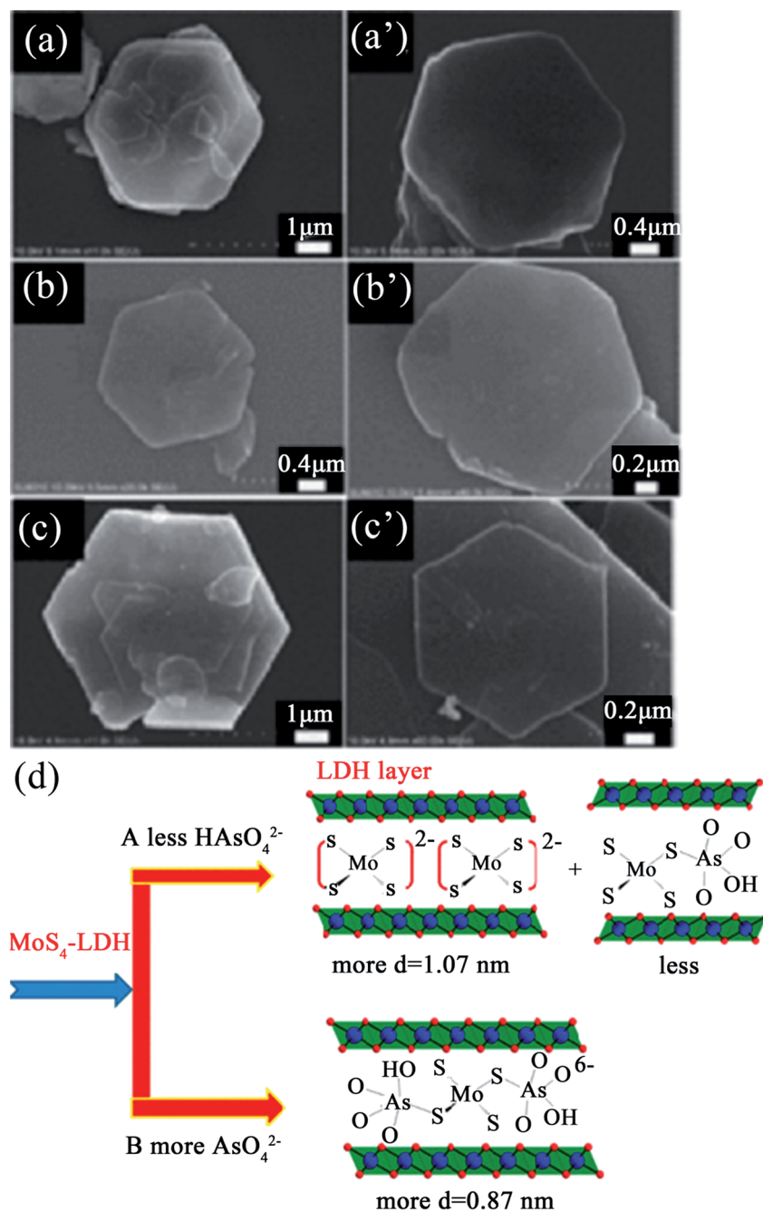
Fig. 6 SEM images of the samples after MoS 4 -LDH adsorption with (a and a') 10 ppm As (iii) , (b and b') 300 ppm As (iii) and (c and c') 10 ppm As (v) ; (d) a scheme showing the dominant phases and possible binding modes of MoS 4 2- with HAsO 4 2- in the LDH gallery (adapted with permission from ref. 89).
