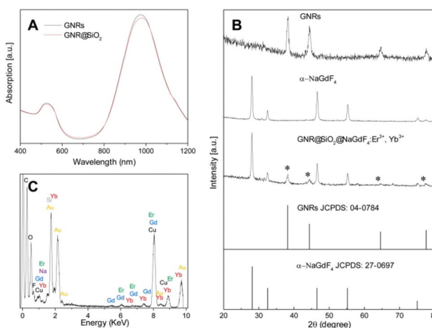
Fig. 2 (A) Extinction spectra of GNRs and GNR@SiO 2 . (B) XRD patterns of GNRs, \alpha -NaGdF 4 :Er 3+ , Yb 3+ , hybrid nanocomposite of GNRs and NaGdF 4 :Er 3+ , Yb 3+ (GNR@SiO 2 @UCNP). The standard pattern of pure GNRs (JCPDS file No: 04-0784), pure \alpha -NaGdF 4 (JCPDS file No: 27-0697) are provided for reference. The stars show the diffraction peaks of GNRs in the GNR@SiO 2 @UCNP nanocomposite. (C) Elemental analysis of hybrid GNRs@SiO 2 @UCNP nanocomposite by EDX.
