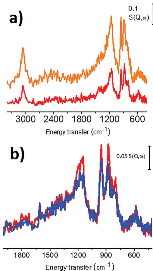
Fig. 5 Part (a) INS spectra of C_w (red spectrum) and C_{\text{Chem}} (orange spectrum). Part (b) INS spectra of C_w (red) and of the corresponding \text{Pd}/C_w catalyst (blue). Previously unpublished figure, reporting data published in ref. 1.
