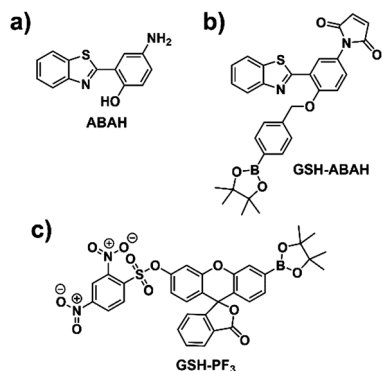
Fig. 1 (a) ABAH ESIPT fluorophore previously used in the literature (b) this work – ESIPT-based probe GSH-ABAH for the detection of ONOO - and biological thiols (c) structure of the GSH-PF 3 probe previously used for the simultaneous detection of ONOO - and GSH.
