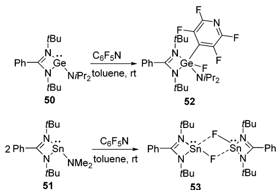
Scheme 18 Activation of C–F bond of C 6 F 5 N by germlyene and stannylene.
