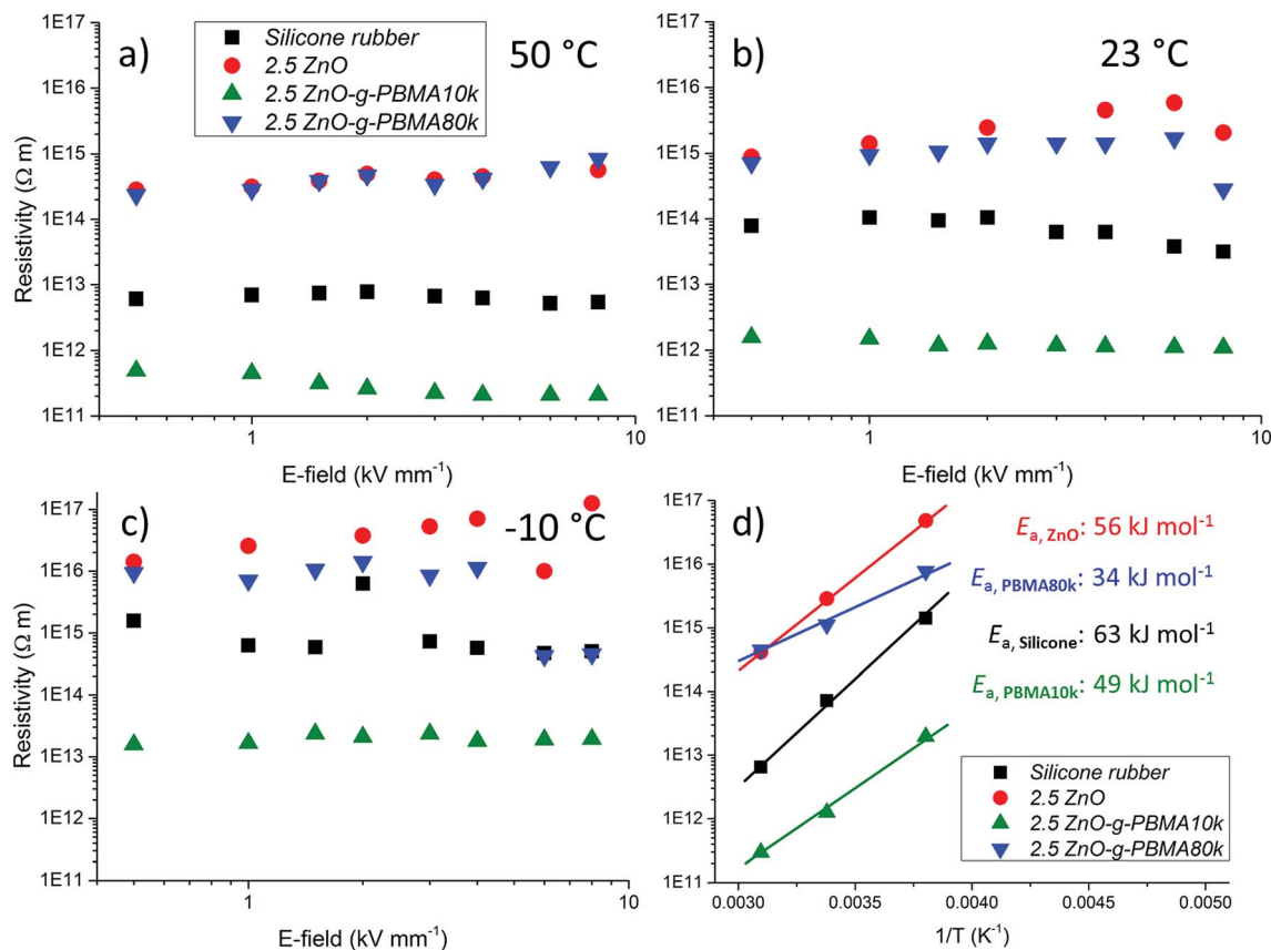
Fig. 14 Resistivity data for silicone rubber, 2.5ZnO, 2.5ZnO- g -PBMA10k and 2.5ZnO- g -PBMA80k at (a) 50 °C, (b) 23 °C and (c) –10 °C. (d) The logarithmic average resistivity plotted against 1/T . Curve fitting gives the slopes corresponding to the temperature dependence of the resistivity and the activation energy of the materials.
