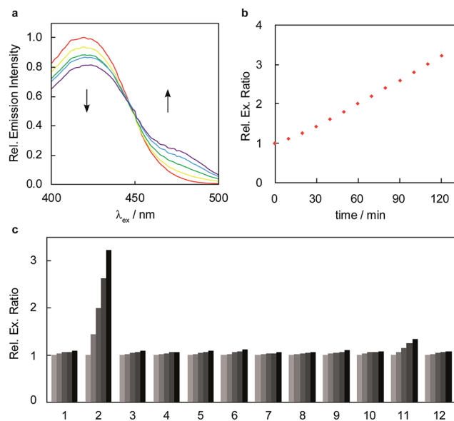
Fig. 2 FA response and selectivity of RFAP-1. Data were acquired at 37^\circ\text{C} in 20 mM PBS (pH 7.4). Excitation spectra were collected between 400 and 500 nm with emission monitored at \lambda_{\text{em}} = 510 nm. (a) Excitation ratiometric response of 10\ \mu\text{M} RFAP-1 to 100\ \mu\text{M} FA. Excitation spectra are shown at 0, 30, 60, 90, and 120 min (red, yellow, green, blue, and purple traces, respectively) after addition of FA. (b) Quantification of 470/420 nm excitation ratio over time. (c) Excitation ratiometric response of 10\ \mu\text{M} RFAP-1 to biologically relevant RCS and related molecules. Bars represent relative 470/420 nm excitation ratios at 0, 30, 60, 90, and 120 (black) min after the addition of a given analyte. The data shown are for a concentration of 100\ \mu\text{M} for all species unless otherwise denoted. Legend: (1) PBS; (2) FA; (3) acetaldehyde; (4) pyruvate; (5) glucose, 1 mM; (6) 4-HNE; (7) dehydroascorbate; (8) oxaloacetate; (9) glucosone; (10) acrolein; (11) methylglyoxal; (12) methylglyoxal, 10\ \mu\text{M} .
