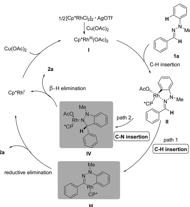
Scheme 4 Proposed mechanism.
