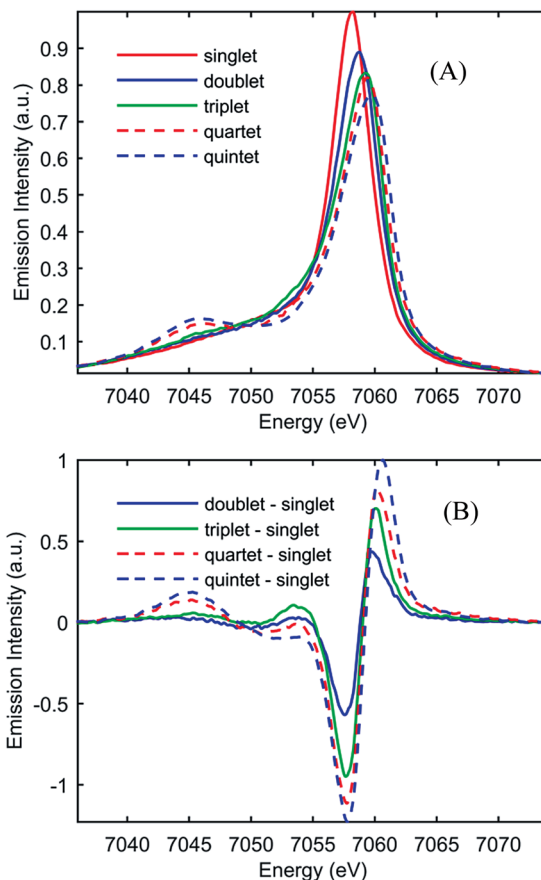
Fig. 2 (A) Model K \beta fluorescence spectra for the ground-state and MLCT, {}^3\text{MC} , {}^5\text{MLCT} , and {}^5\text{MC} excited states of [\text{Fe}(\text{CN})_4(\text{bpy})]^{2-} . The model spectra are constructed from ground-state iron complexes with different spin moments; singlet: linear combination of [\text{Fe}(\text{bpy})_3]^{2+} and [\text{Fe}(\text{CN})_6]^{4-} (red), doublet: linear combination of [\text{Fe}(\text{bpy})_3]^{2+} and [\text{Fe}(\text{CN})_6]^{3-} (blue), triplet: iron(II)phthalocyanine (green), quartet: iron(III)phthalocyanine (dashed red), and quintet [\text{Fe}(\text{phenanthroline})_2(\text{NCS})_2] (dashed blue). (B) Reference difference K \beta spectra for the MLCT, {}^3\text{MC} , {}^5\text{MLCT} , and {}^5\text{MC} excited states constructed from the ground-state model spectra by subtracting the singlet spectrum. For detailed discussion of the modeling of the difference spectra, see the ESI.†
