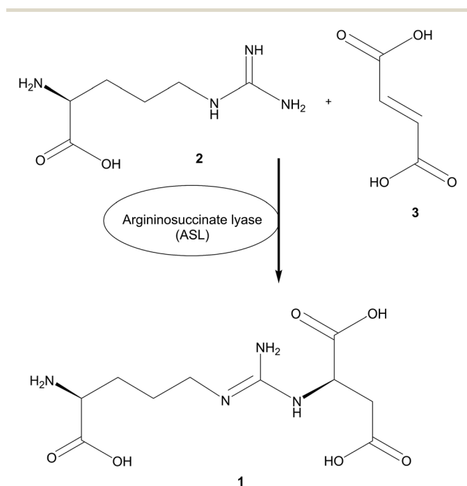
Fig. 1 Argininosuccinate lyase-catalyzed reaction between L -arginine 2 and fumarate 3 to N -(((4 S )-4-amino-4-carboxybutyl]amino)iminomethyl)- L -aspartate 1 (in short: L -argininosuccinate) as part of the urea cycle running in reverse.
