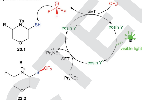
Scheme 23 Trifluoromethylation of disubstituted morpholines.
