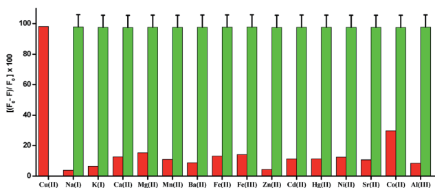
Fig. 4 Fluorescence Quenching Efficiency (FQE) of H 5 dpm (5 × 10 -6 M) in Tris buffer solution (25 mM, pH = 7.4) in the presence of 100 μM of different types of metal ions except Cu 2+ (50 μM) as a bar graph [the red bar portion]. Fluorescence Quenching Efficiency (FQE) of a mixture of H 5 dpm (5 × 10 -6 M) solution with other metal ions (100 μM) followed by addition of 50 μM Cu 2+ to the solution [the green bar portion] (λ ex = 434 nm, λ em = 510 nm, slit: 5 nm/5 nm).
