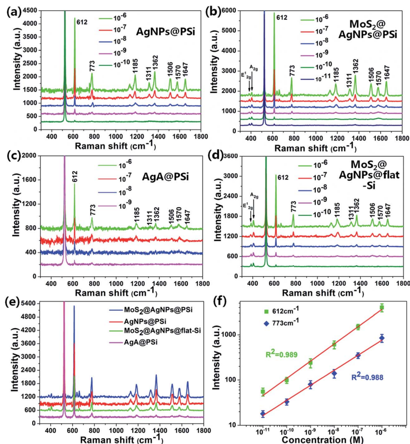
Fig. 5 (a) The Raman spectra of R6G on the AgNPs@PSi substrate from 10^{-6} to 10^{-10} M. (b) The Raman spectra of R6G on the \text{MoS}_2@AgNPs@PSi substrate from 10^{-6} to 10^{-11} M. (c) The Raman spectra of R6G on the AgA@PSi substrate from 10^{-6} to 10^{-9} M. (d) The Raman spectra of R6G on the \text{MoS}_2@AgNPs@flat-Si substrate from 10^{-6} to 10^{-10} M. (e) The Raman spectra of R6G on the \text{MoS}_2@AgNPs@PSi , AgNPs@PSi, \text{MoS}_2@AgNPs@flat-Si and AgA@PSi substrates with concentration of 10^{-6} M. (f) Raman intensity of R6G at 612 and 773 \text{cm}^{-1} as a function of the molecular concentration on the \text{MoS}_2@AgNPs@PSi substrate, in log scale.
