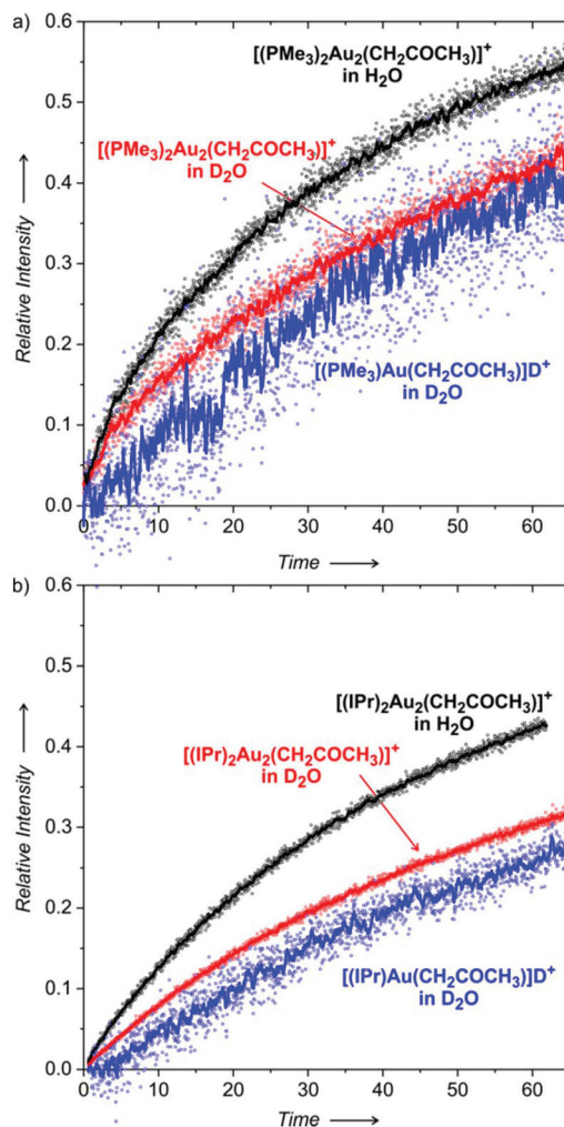
Fig. 8 Time evolution of the relative concentration of [(\text{L})_2\text{Au}_2(\text{CH}_2\text{COCH}_3)]^+ (L is (a) \text{PMe}_3 or (b) IPr) with respect to the sum of [(\text{L})_2\text{Au}_2(\text{CH}_2\text{COCH}_3)]^+ and [(\text{L})_2\text{Au}_2(\text{CD}_2\text{COCD}_3)]^+ in a solution with 33% \text{H}_2\text{O} (in black) or 33% \text{D}_2\text{O} (in red). The blue points show the corrected evolution of \text{D}^+ tagged neutral [(\text{L})\text{Au}(\text{CH}_2\text{COCH}_3)] with respect to \text{D}^+ tagged [(\text{L})\text{Au}(\text{CD}_2\text{COCD}_3)] under the assumption that the concentrations of [(\text{L})\text{Au}(\text{CH}_3\text{COCH}_3)]^+ and [(\text{L})\text{Au}(\text{CD}_3\text{COCD}_3)]^+ are equal (see the text). Experiments: (a) [(\text{PMe}_3)\text{AuSbF}_6] (77 \mu\text{g} ) was dissolved in THF (0.8 ml), \text{CD}_3\text{COCD}_3 (0.4 ml), and \text{H}_2\text{O} or \text{D}_2\text{O} (0.6 ml) and left to react for 15 hours. Then, 0.4 ml of \text{CH}_3\text{COCH}_3 was added and the solution was immediately monitored by ESI-MS. (b) [(\text{IPr})\text{AuBF}_4] (358 \mu\text{g} ) was dissolved in dioxane (0.2 ml), \text{CD}_3\text{COCD}_3 (0.7 ml) and \text{H}_2\text{O} or \text{D}_2\text{O} (0.45 ml) and left to react for 15 hours. Then, 0.7 ml of \text{CH}_3\text{COCH}_3 was added and the solution was immediately monitored by ESI-MS. The lines correspond to 10 points smoothing.
