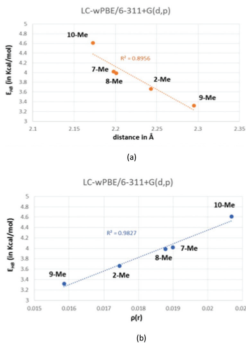
Fig. 7 Correlation between the calculated energy of the hydrogen bond ( E_{HB} ) and either the O...Ha distance (a) or the charge density (b).
