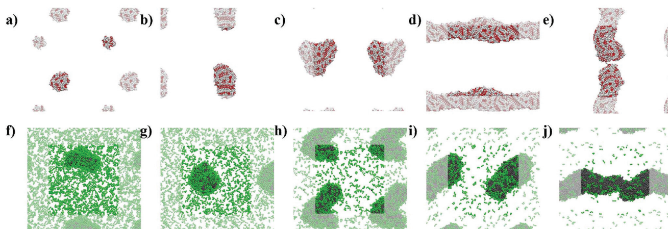
Fig. 3 Simulation snapshots at 10 \mu\text{s} for: (a) F_6^{100} , (b) F_6^{200} , (c) F_6^{300} , (d) F_6^{400} , (e) F_6^{500} , (f) F\text{-}L^{100-1500} , (g) F\text{-}L^{200-1200} , (h) F\text{-}L^{300-900} , (i) F\text{-}L^{400-600} and (j) F\text{-}L^{500-300} . (a–e) F_6 systems show backbone beads in red and side chain beads in white; (f–j) and F\text{-}L systems show F_6 molecules in grey and L_2 in green. Periodic images are transparent for all the systems.
