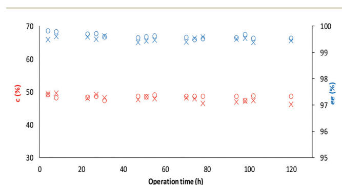
Fig. 8 Long term stability of the CaLB entrapped in the TDP sol-gel system in KR of the alcohol rac-1a ( c\% : x, ee_{(R)-2a} : o) and amine rac-3a ( c\% : o, ee_{(R)-4a} : x) in a continuous-flow reactor (60 °C, flow-rate of 0.1 mL min -1 ).
