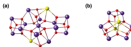
Fig. 8 Cores of polynuclear complexes by Mishra et al. 175 (a) and by Chen et al. 177 (b) containing \text{Mn}_3\text{Ca} cubanes as integrated substructures (ligands omitted for clarity).
