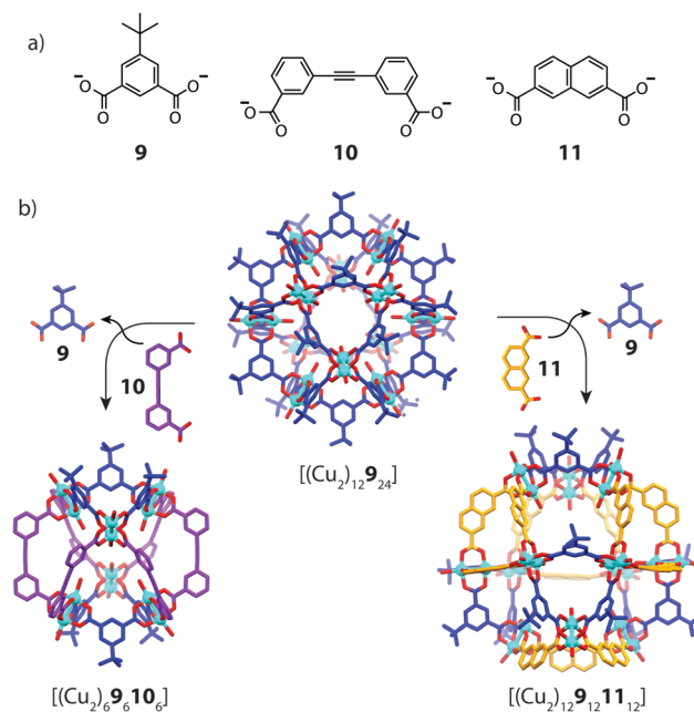
Fig. 7 (a) Bent dicarboxylate ligands 9–11 bearing angles of 120°, 60° and 120° respectively; (b) transformation of the homoleptic [(Cu_2)_{12} 9_{24}] cage to heteroleptic species [(Cu_2)_6 9_6 10_6] (left) and [(Cu_2)_{12} 9_{12} 11_{12}] (right) by ligand substitution.
