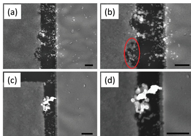
Fig. 3 SEM image taken after 10^2 consecutive I-V sweeps for (a) Ag/Ag-PEO/Pt and (c) Ag/PEO/Pt planar devices with a gap distance of \sim 1 and \sim 0.5 \mu\text{m} , respectively. The left and right electrodes correspond to Ag and Pt, respectively. Images (b) and (d) are the corresponding magnified views. I_{CC} was set at 1 mA and 400 \mu\text{A} for the Ag-PEO and PEO devices, respectively. The scale bar is 500 nm.
